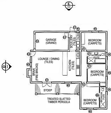
PLAN - HOUSE 1:100
